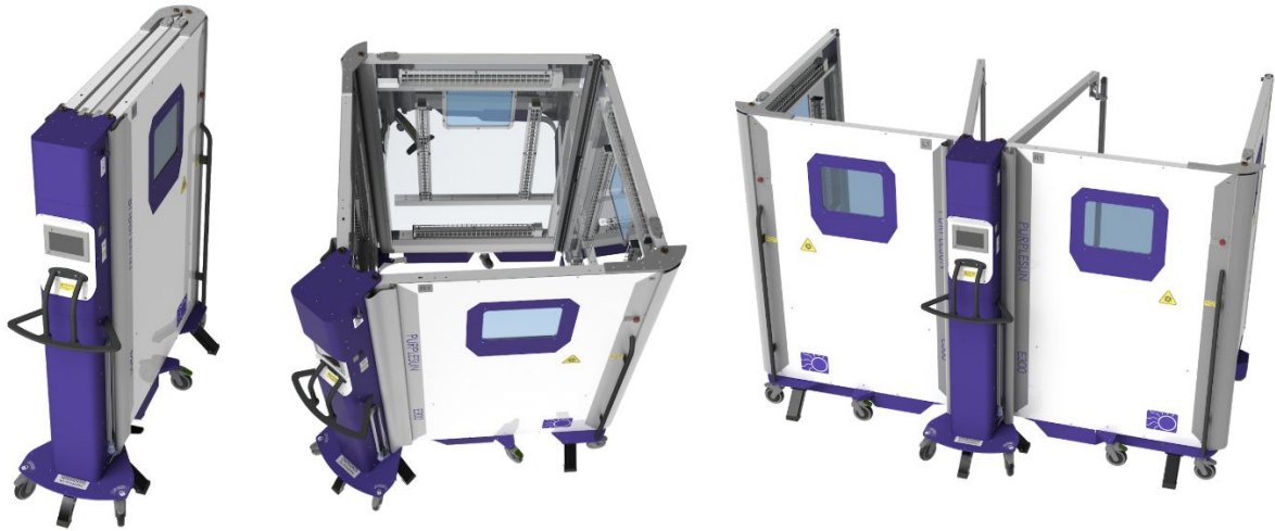
Figure 1: The PurpleSun E300 FMUV system in PACT configuration for transport or storage (Left), CUBE configuration for surrounding smaller equipment (Center), and RECTAN mode for surrounding larger equipment (Right).
